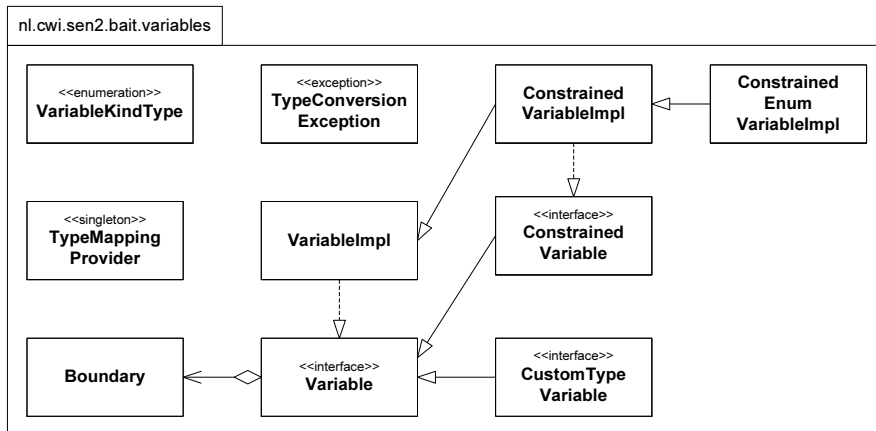
Figure 5.5: Package nl.cwi.sen2.bait.variables
