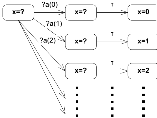
Figure 2.6: The LTS of the simple system
