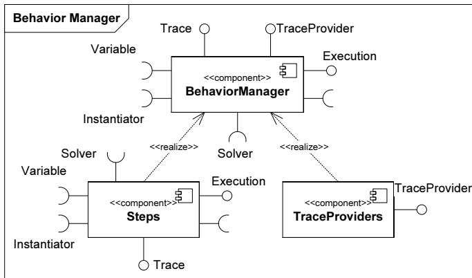
Figure 5.7: Component BehaviorManager
