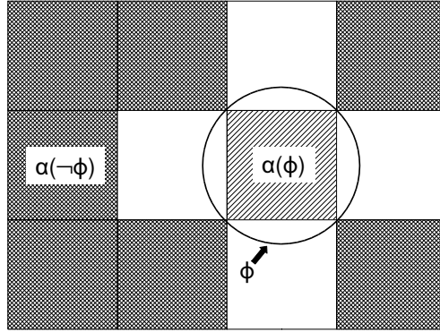
Figure 7.4: Contracting abstraction
