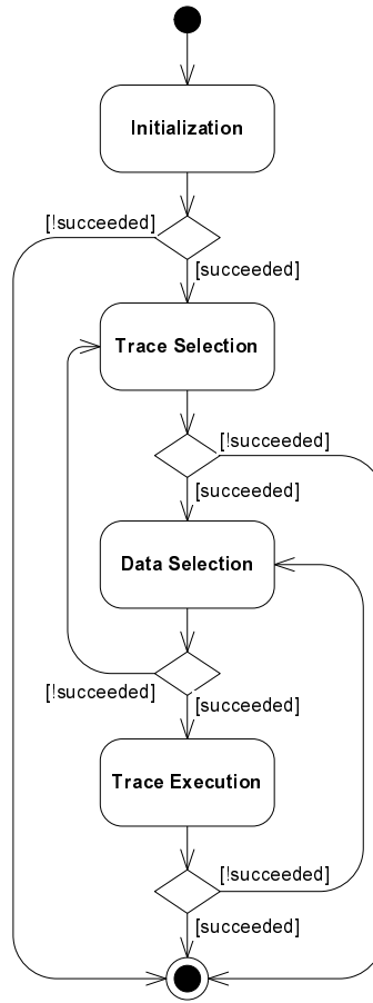
Figure 5.10: The test execution process
