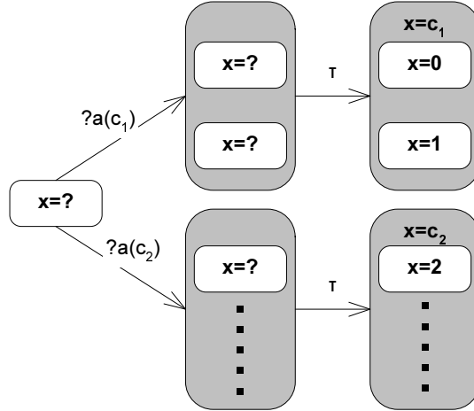
Figure 2.7: The LTS of the abstracted simple system
