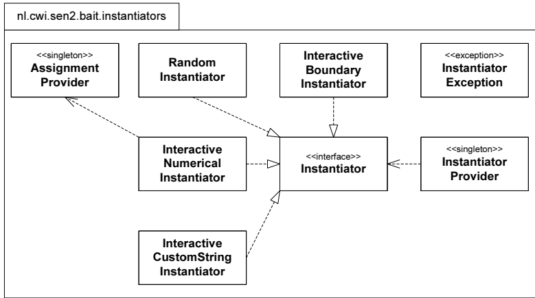
Figure 5.6: Package nl.cwi.sen2.bait.instantiators
