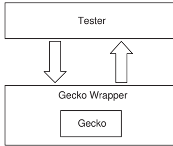
Figure 6.7: Test environment
