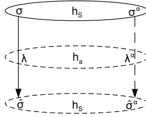
Figure 7.3: Abstraction requirement for LTSs
