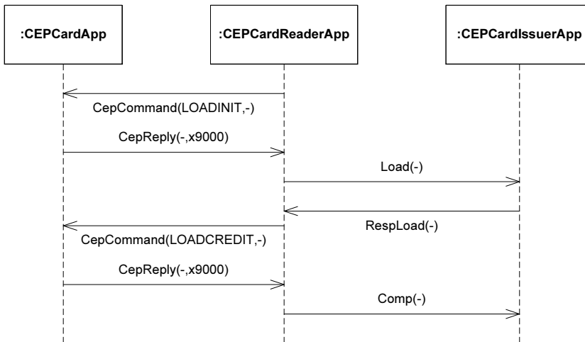
Figure 4.6: Interactions in the test purpose scenario
