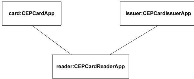
Figure 4.5: Collaborating system roles in CEPS
