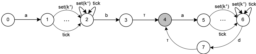
Figure 7.9: The violation pattern for the counterexample
