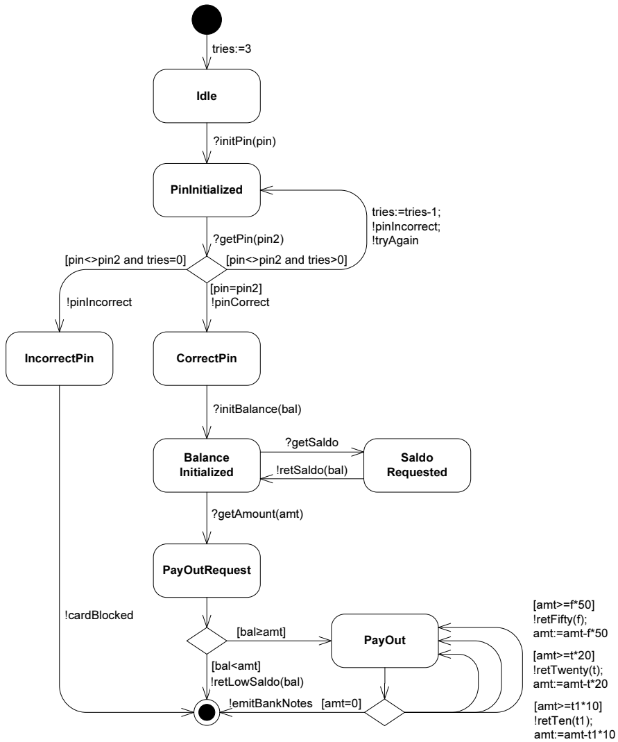
Figure 6.2: Specification of the ATM
